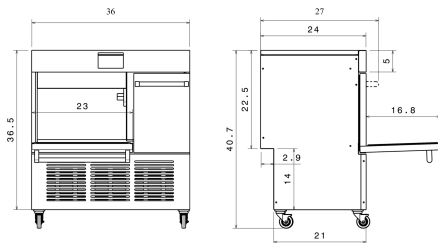
FRONT VIEW | SIDE VIEW — Dimensions in inches
