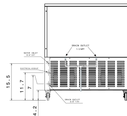
REAR UTILITY CONNECTIONS — Dimensions in inches
